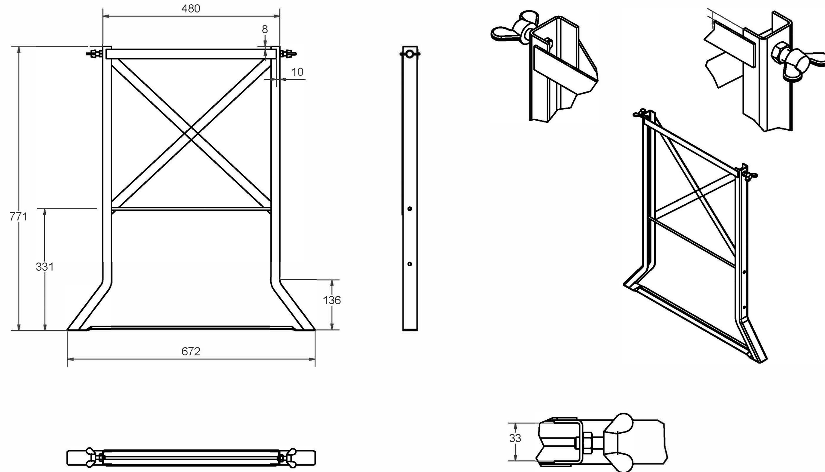
TECHNICAL DRAWING OF 30000
